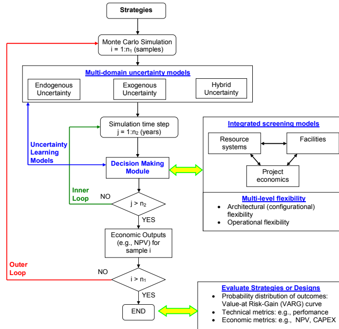
Fig. 2. A computational framework to explore flexibility under multi-domain uncertainty, i = sample in uncertainty space, j = time step index, n_1 =number of Monte Carlo samples, n_2 = number of total time steps.
